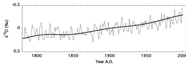
Figure 10. Fiji coral \delta^{18}\text{O} composite made from the arithmetic average of the five individuals coral records (thin black line) and its extracted secular trend (SSA frequency lower than 75 years) (bold black line).
