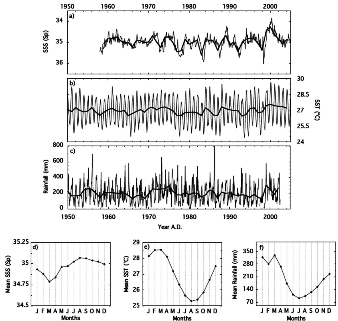
Figure 2. Gridded monthly (thin) and annually averaged (bold) Fiji climatology (a) sea surface salinity (Sp) centered on 17°S–179°E and extending from January 1958 to December 2004 [Delcroix et al., 2011], (b) ERSST Sea Surface Temperature (°C); data set centered on 178°W–18°S extending from January 1950 to December 2004 (LDEO Climate Data Library: http://iridl.ldeo.columbia.edu/SOURCES/.NOAA/.NCDC/.ERSST/.version3/.SST/ ) [Smith et al., 2008], and (c) cumulative precipitation (mm) from various sites around Fiji from January 1950 to July 2002 (PACRAIN database retrieved from http://pacrain.evac.ou.edu ). The long-term Fiji climatology (d) SSS, (e) SST, and (f) precipitation, over the common period of the three data sets (1958 to 2002).
